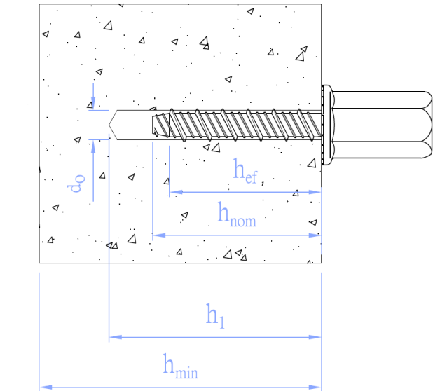
Drawing A2. Installed condition for anchors AMDTH, AMROD, AMROF, AMROH, AMRHH, AMROO, AMRCC, AMRHC and AMROC.
